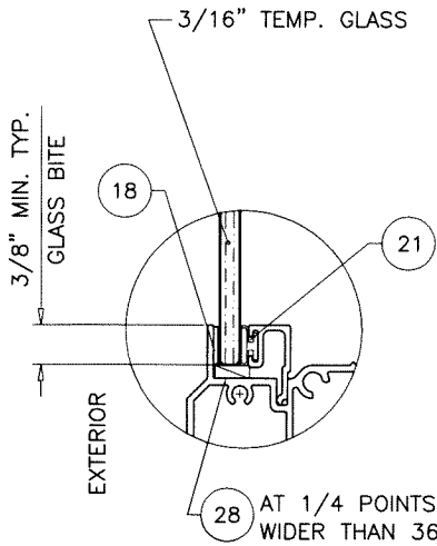
GLASS TYPE 'A' 3/16" TEMP. GLASS
