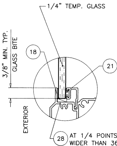
GLASS TYPE 'C' 1/4" TEMP. GLASS
