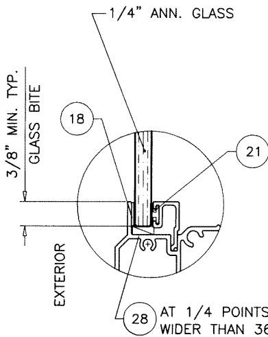
GLASS TYPE 'B' 1/4" ANN. GLASS
